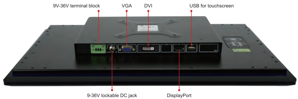
DM-F19A Fully Integrated I/O
